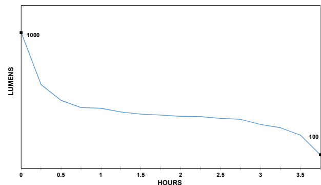
PERFORMANCE CURVE
